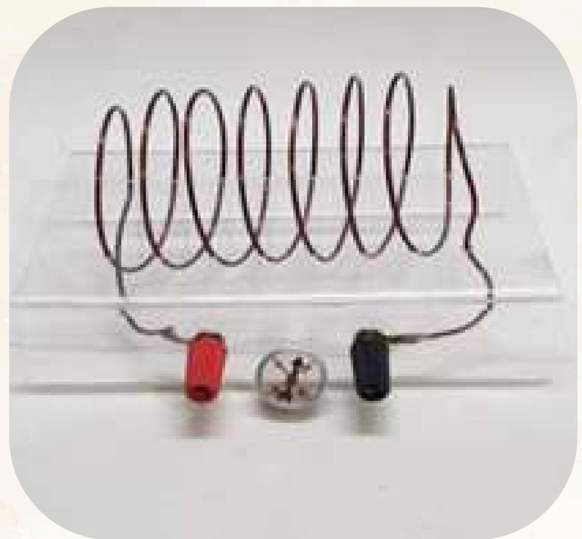
MAGNETIC FIELD DEMONSTRATION
